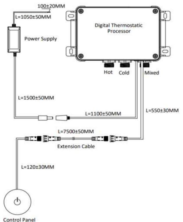
System Connection Diagram
