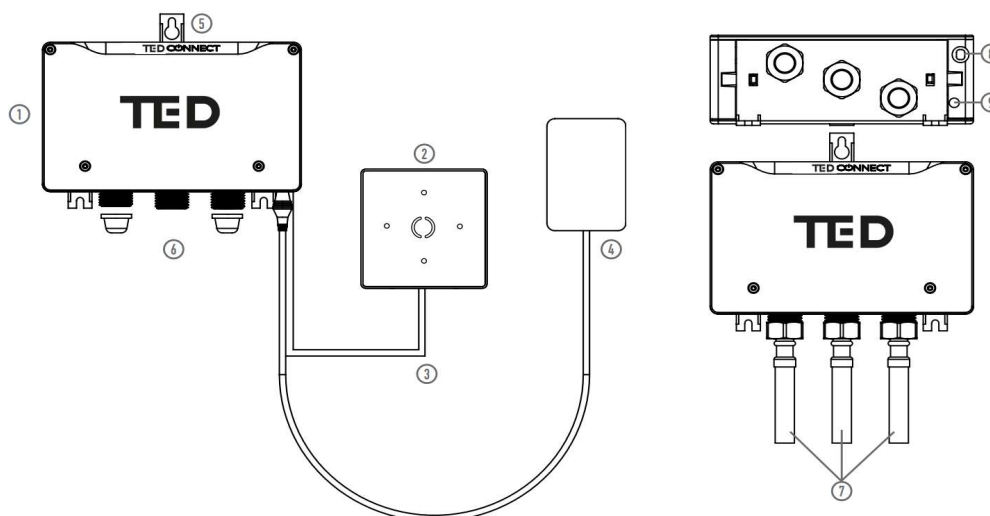
Connection Schematic
