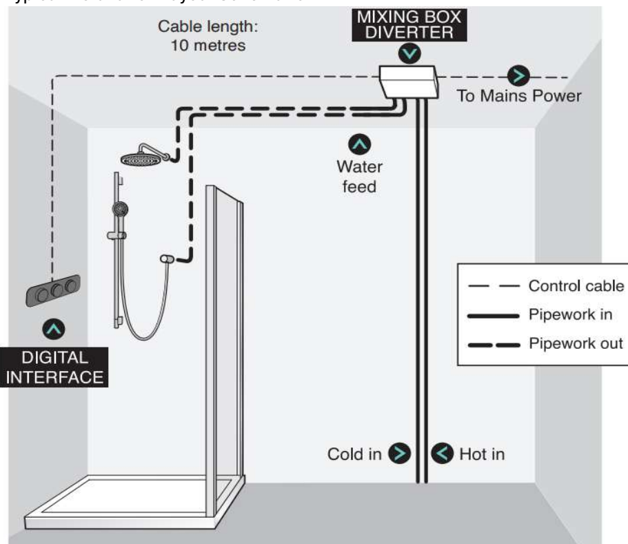
Typical Installation Layout Schematic
