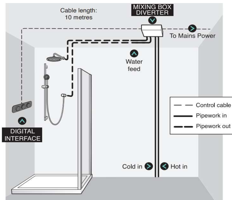
Connection Diagram
